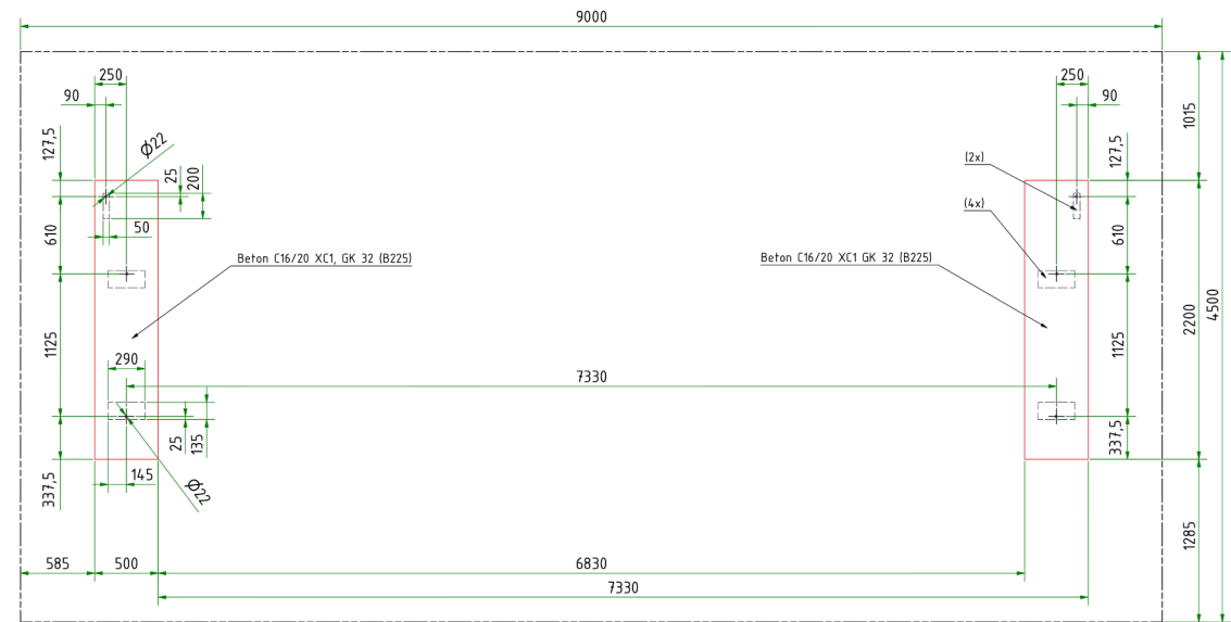
Fundamentplan:
