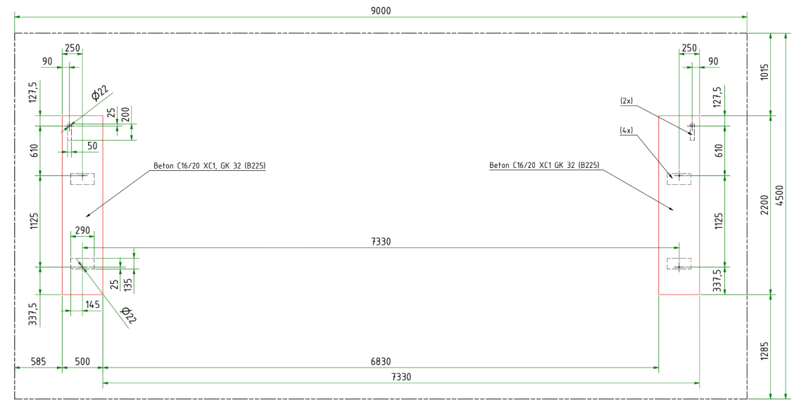
Fundamentplan:
