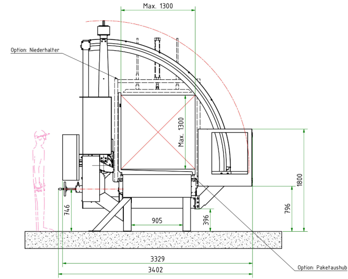
Fundamentplan:
