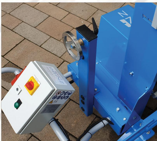
Side shift mechanism (optional)
